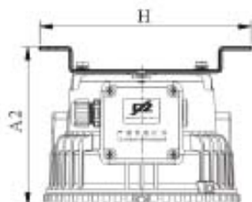
Ceiling Bracket
