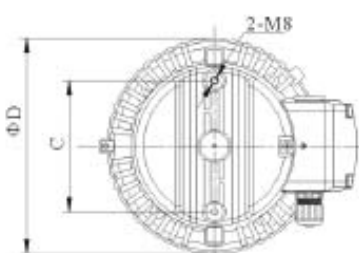
Trunnion bracket
