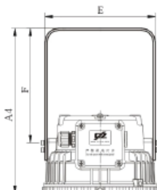
Trunnion bracket
