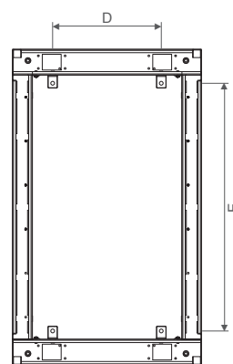
Base View
