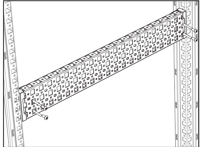
11-1-12 Fixing Method 1
