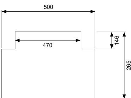
Rebate dimensions
