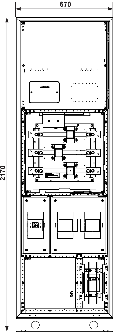
Front View
