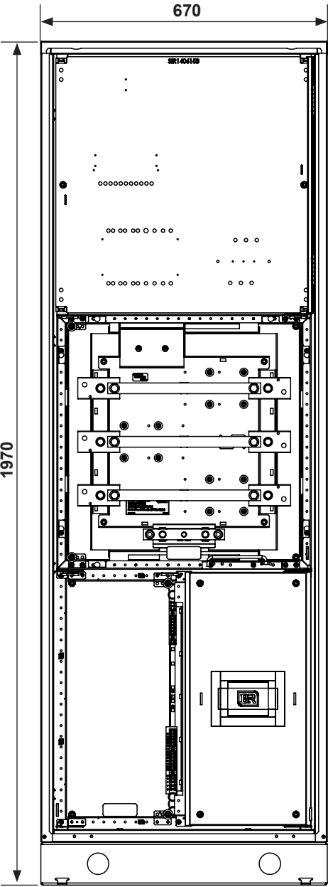
Front View
