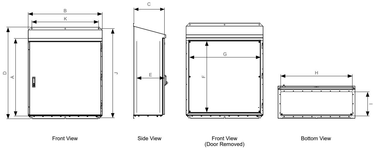
Internal Enclosure
